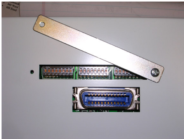
Figure A: removing the DIP switch cover at the rear of the control panel
