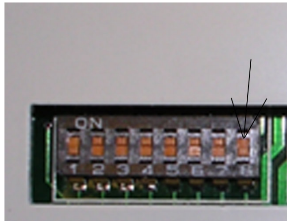
Figure B: DIP switch #8 (indicated by arrow) on the left-side bank of DIP switches
